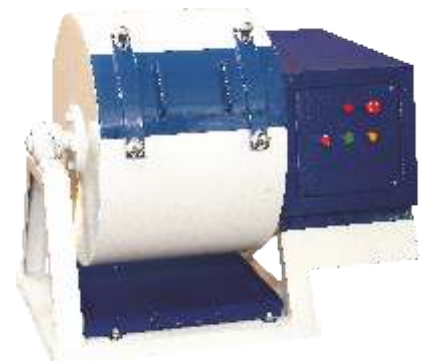
Los Angeles Abrasion Testing Machine
